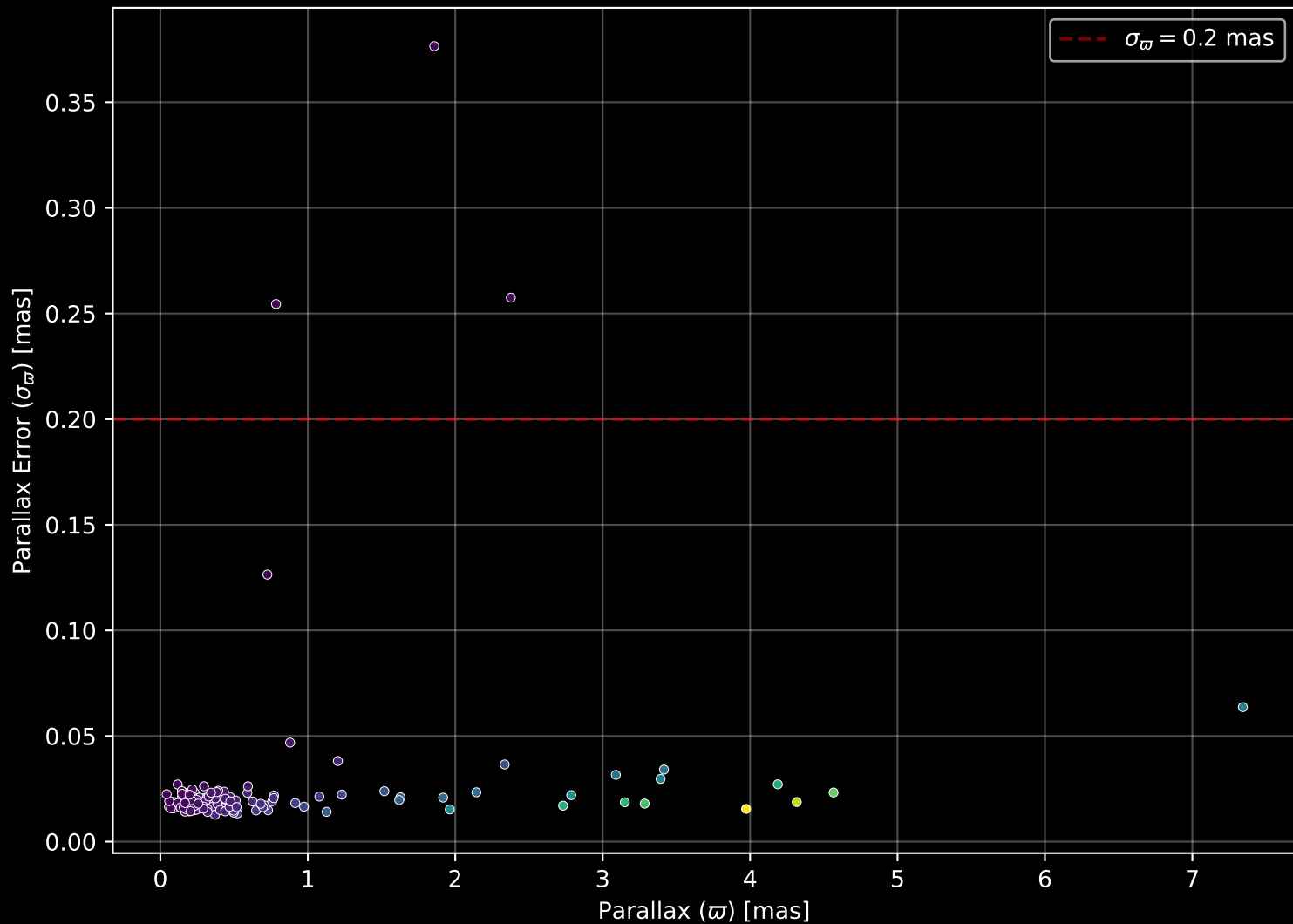
APOGEE DR17 Field: [125-12] Parallax Quality (n= 138)
