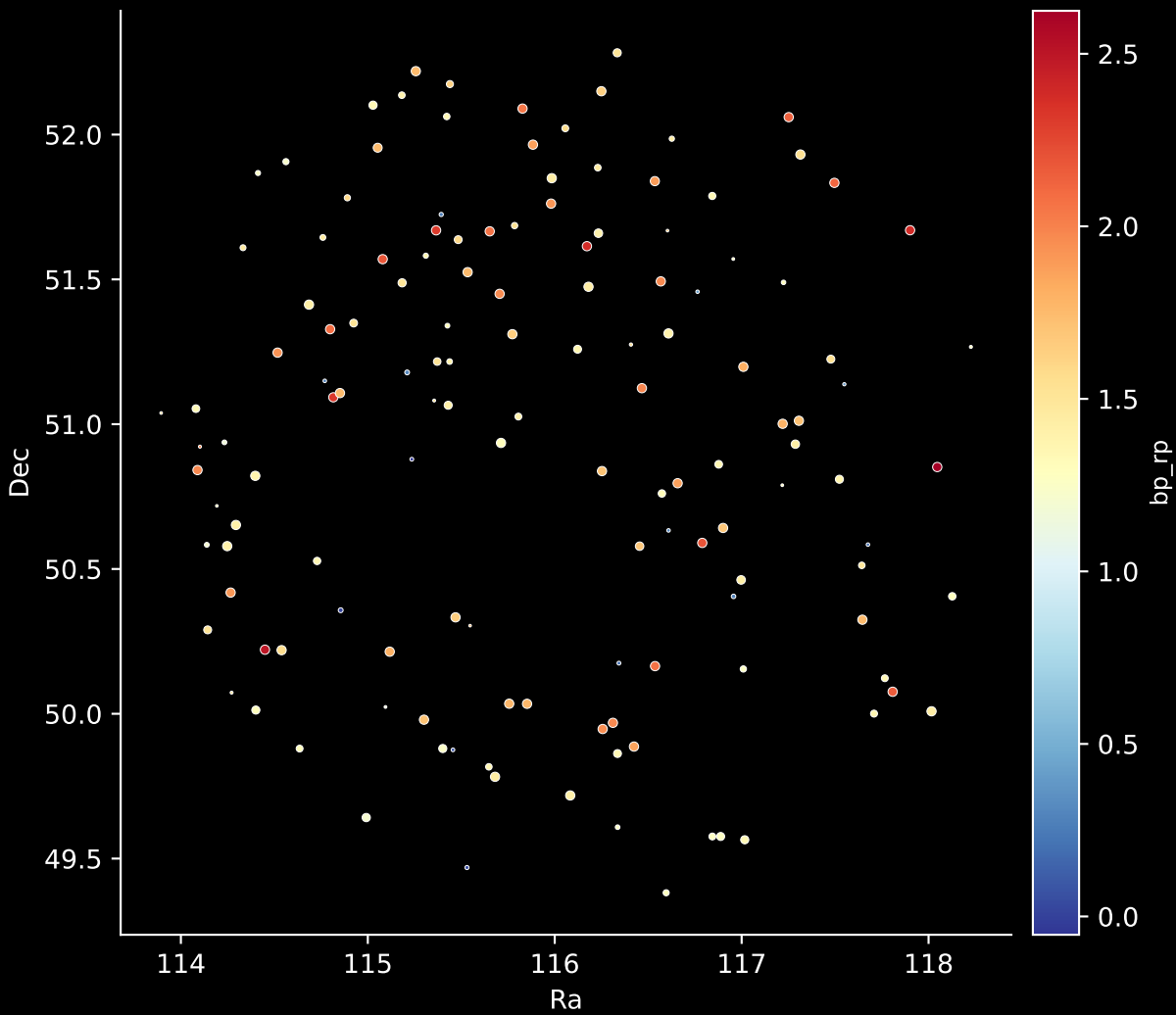
APOGEE DR17 Field: [125-12] Stars: 138
