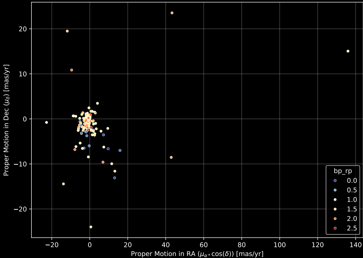
APOGEE DR17 Field: [125-12] Proper Motion Diagram (n= 138)
