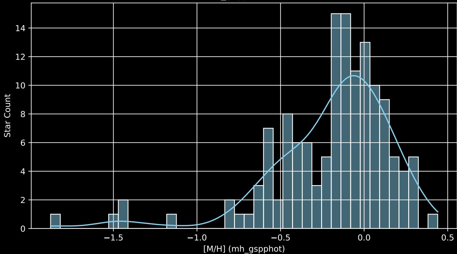
APOGEE DR17 Field: [125-12 [M/H] (mh_gspphot) (n= 137)
