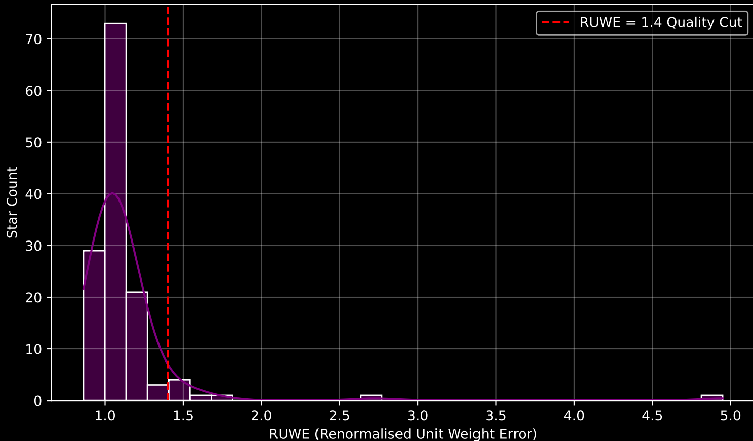
GAPOGEE DR17 Field [125-12] RUWE Distribution (n= 134)
